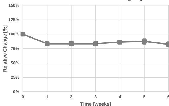
Flexural Stress at Break after UV Ageing
